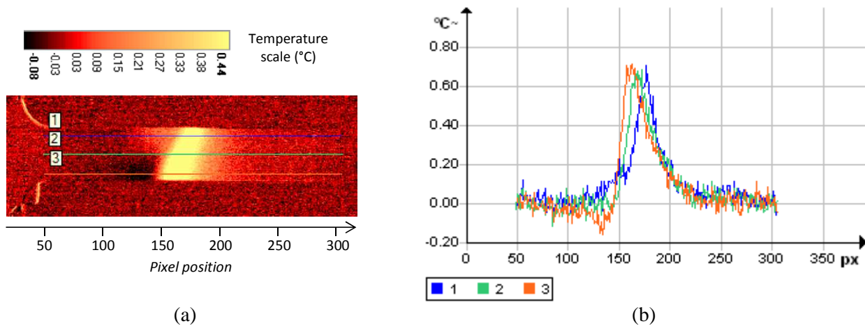
Figure 3. (a) Typical recomputed image (differences between two original images separated of 0.6 s) obtained during Lüders band propagation in a S235 steel. (b) Temperature profiles along three lines uniformly distributed through the specimen width (see (a)).
