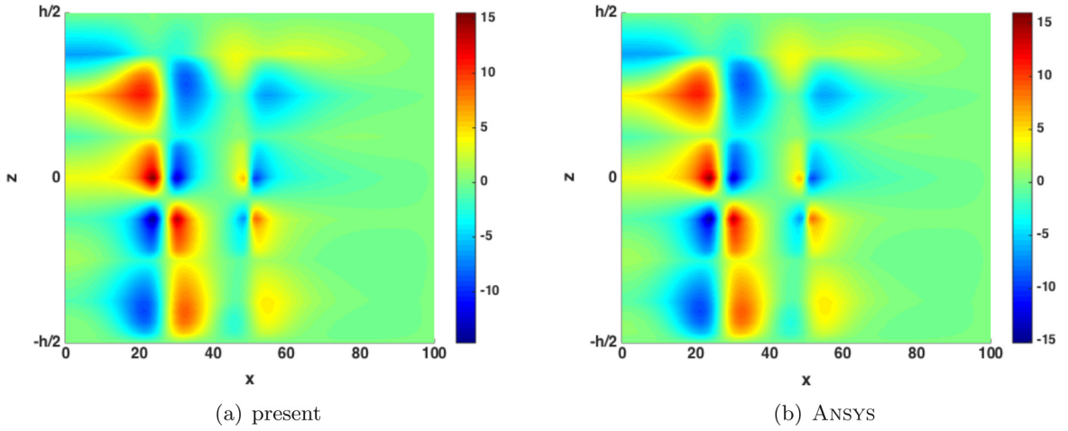
Fig. 23. Distribution of \bar{\sigma}_{13} (different scale for x and z-axis) - 8 layers - 10 couples.
