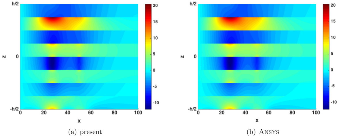
Fig. 22. Distribution of \bar{\sigma}_{11} (different scale for x and z-axis) - 8 layers - 10 couples.
