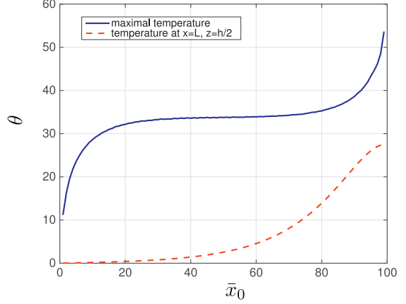
Fig. 18. Distribution of the temperature with respect to the position of the heat source \bar{x}_0 (right) and also along the thickness at x = L (left) - 8 layers.
