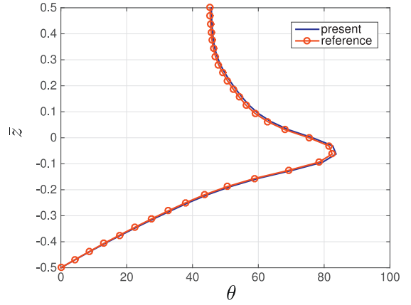
Fig. 19. Distribution of the temperature along the length of the beam at z = 0 (left) and along the thickness at the middle of the interval I_1^{4th} (right) - 8 layers.
