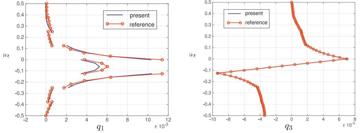
Fig. 20. Distribution of heat flux q_1 at x = 30 (left) and q_3 at the middle of the interval l_1^{4th} (right) along the thickness - 8 layers.
