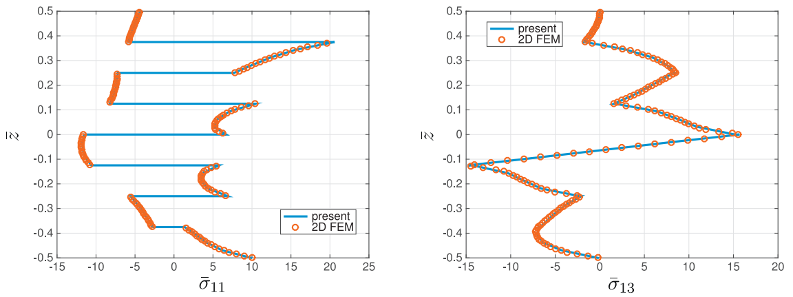
Fig. 24. Distribution of \bar{\sigma}_{11} at x = 28 (left) and \bar{\sigma}_{13} at x = 24 (right) along the thickness - S=10 - 8 layers - 10 couples.
