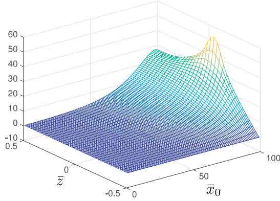
Fig. 18. Distribution of the temperature with respect to the position of the heat source \bar{x}_0 (right) and also along the thickness at x = L (left) - 8 layers.
