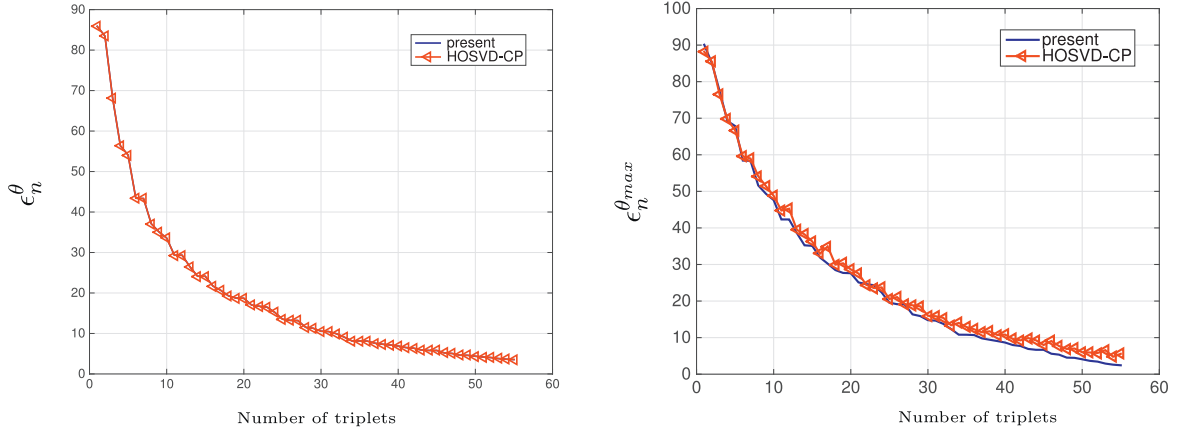
Fig. 15. global error rate (left) - \theta_{max} error rate (right) - comparison between present approach and HOSVD-CP.
