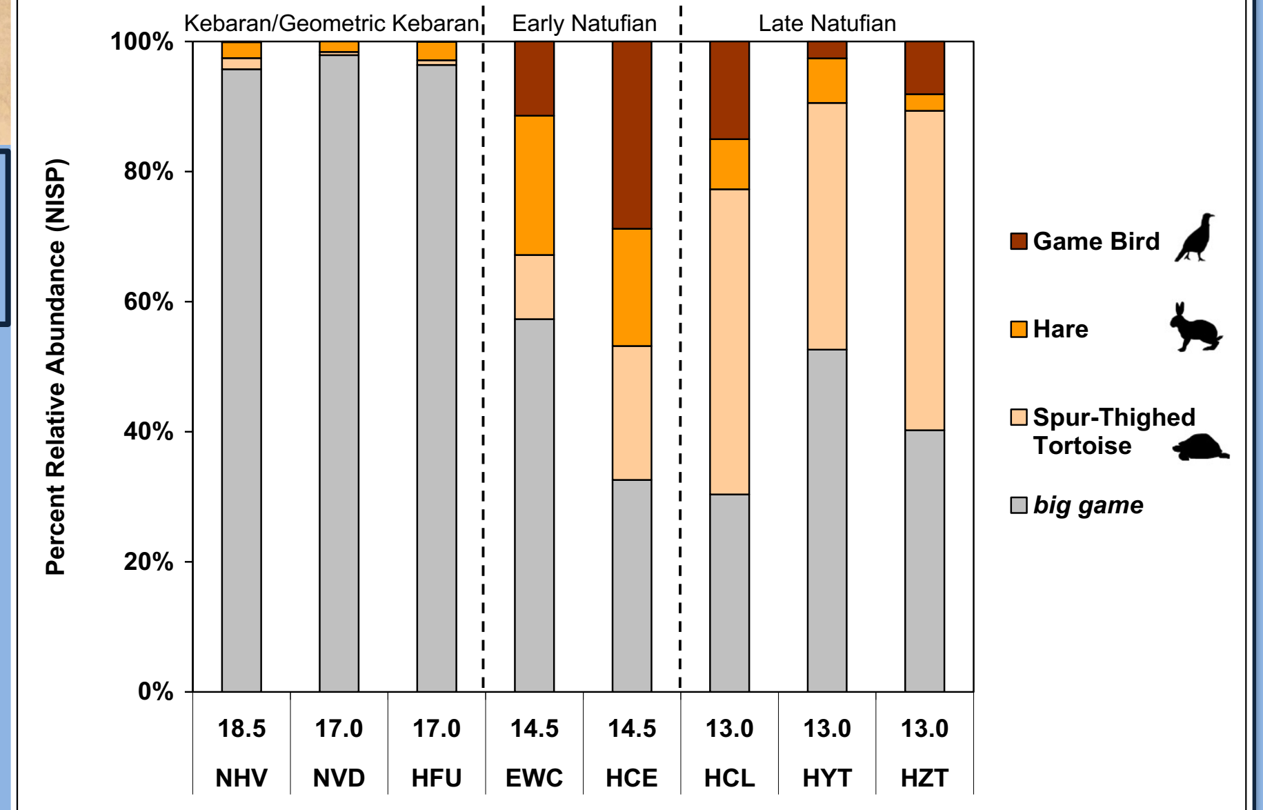
Time-series change in eight faunal assemblages, from Early-Middle Epipaleolithic (Kebaran/Geometric Kebaran) to Early Natufian and Late Natufian periods (ages shown in kya, site codes and data from Stutz et al. 2009). Shown are the rise and fluctuations in small game foraging.
