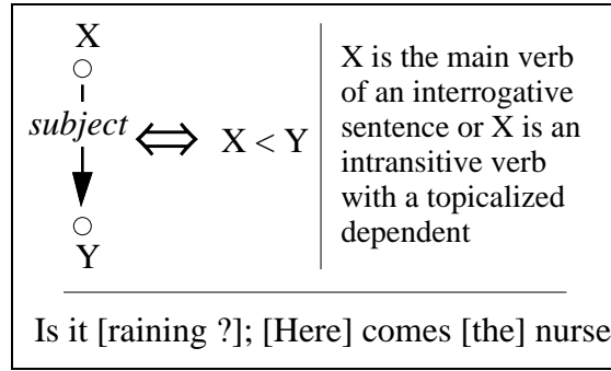
Fig. 11. Two English sagittal surface-syntactic rules
