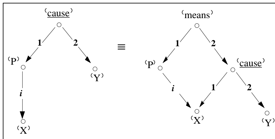
Fig. 4. A rule of equivalence which is not a rule of decomposition
