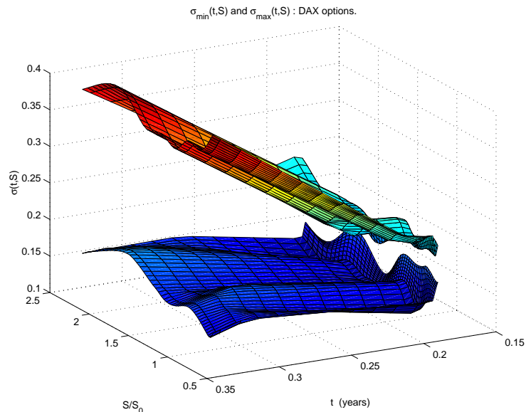
Figure 13: Pointwise confidence intervals for the local volatility \sigma(t, S) computed from 10 best solutions, DAX options.
