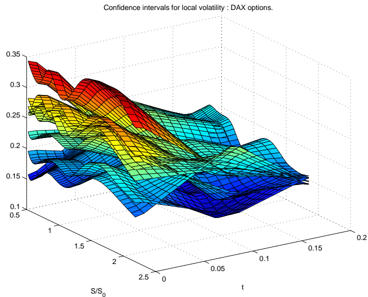
Figure 12: A sample of local volatility surfaces calibrated to DAX options.
