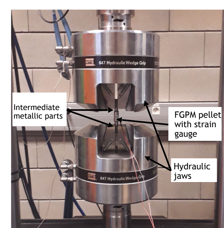
Compression test using an hydraulic Fatigue Testing System
