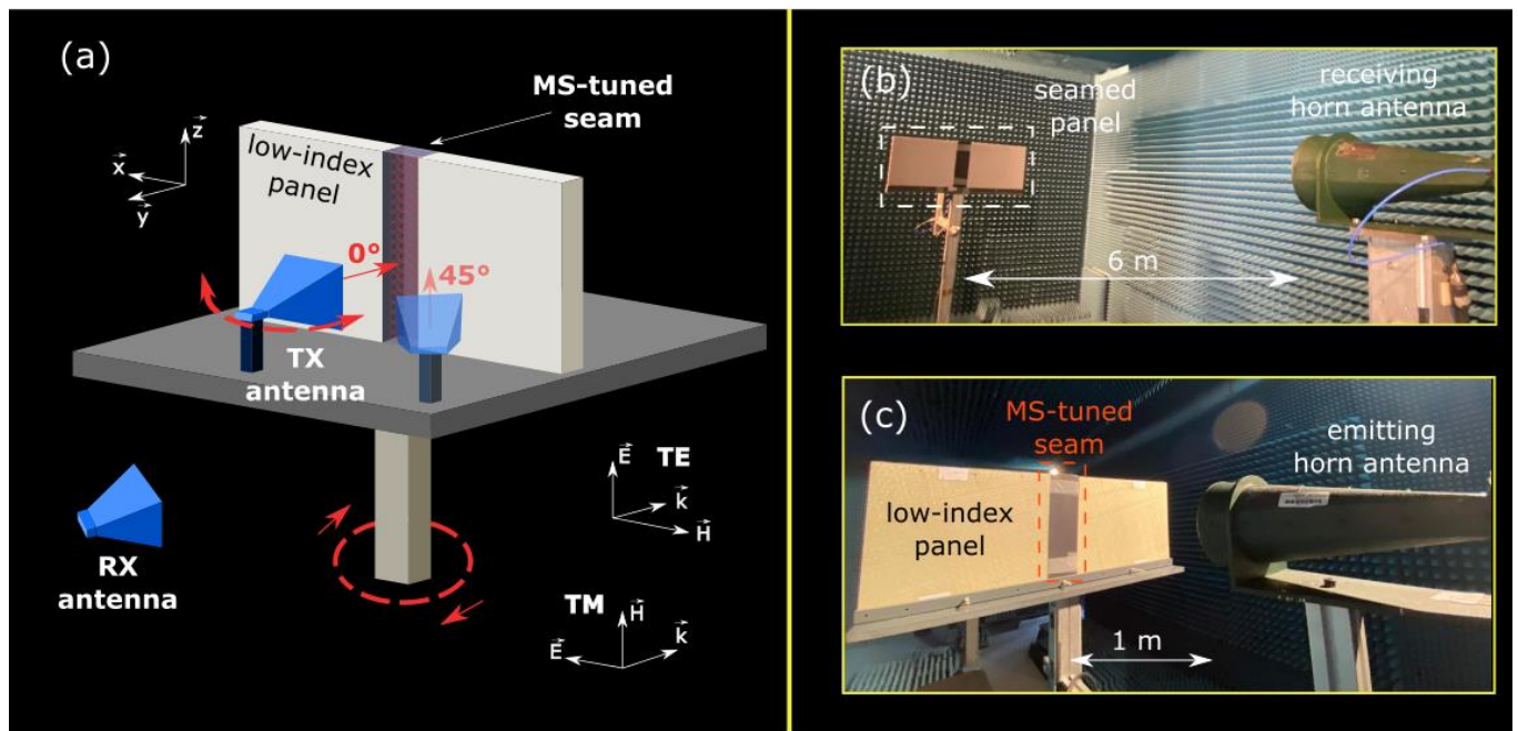
Figure 4. (a) Schematic illustration of the studied structure. Two low-index radome panels are connected via a high-index MS-tuned seam. The structure is illuminated by an emitting (Tx) antenna and a receiving (Rx) antenna allows us to measure the antenna radiation patterns for different angles of incidence. (b) Photography of the far-field measurement setup in an anechoic chamber. (c) Close up of the emitting antenna illuminating the seamed panel.
