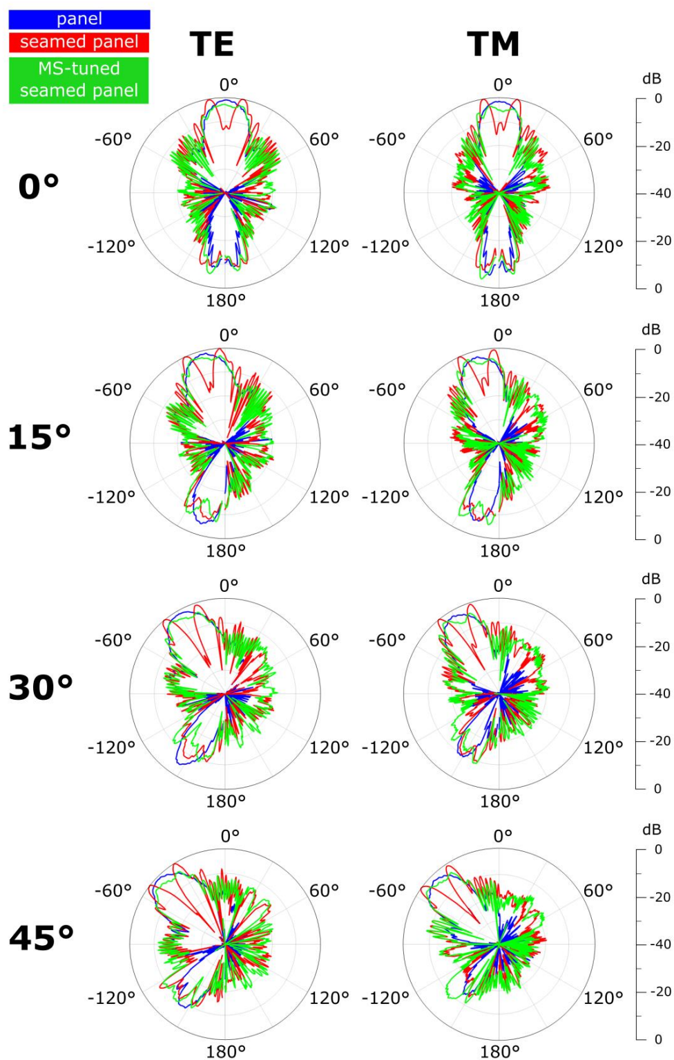
Figure 5. Measured far-field radiation patterns in the case of the reference panel (blue), the seamed panel without MSs (red) and the MS-tuned seamed panel (green), for 0°-, 15°-, 30°-, and 45°-incident, TE- (first column) and TM-polarized (second column) illuminations at 10.5 GHz.
