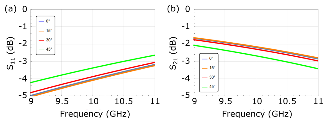
Figure 2. Evolution of the S-parameters of the optimized unit cell as a function of frequency for 0^\circ, 15^\circ, 30^\circ , and 45^\circ obliquely incident illuminations. (a) S_{11} and (b) S_{21} . The S-parameters are obtained by simulating the optimized unit cell with Floquet ports and periodic boundary conditions.
