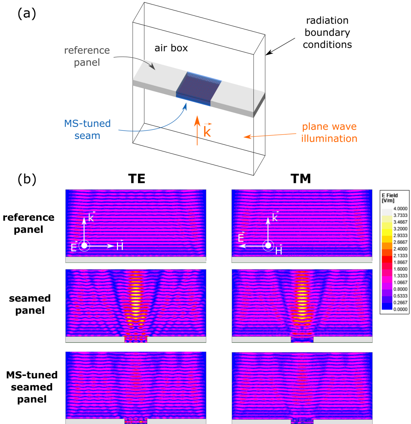
Figure 3. Numerical validation of the camouflaging effect. (a) Simulation setup, where a plane wave is used to illuminate the structure. (b) Scattered field distributions in the case of normally incident TE- and TM-polarized plane waves illuminating the reference panel (first row), the non-tuned seamed panel (second row) and the MS-tuned seamed panel (third row).
