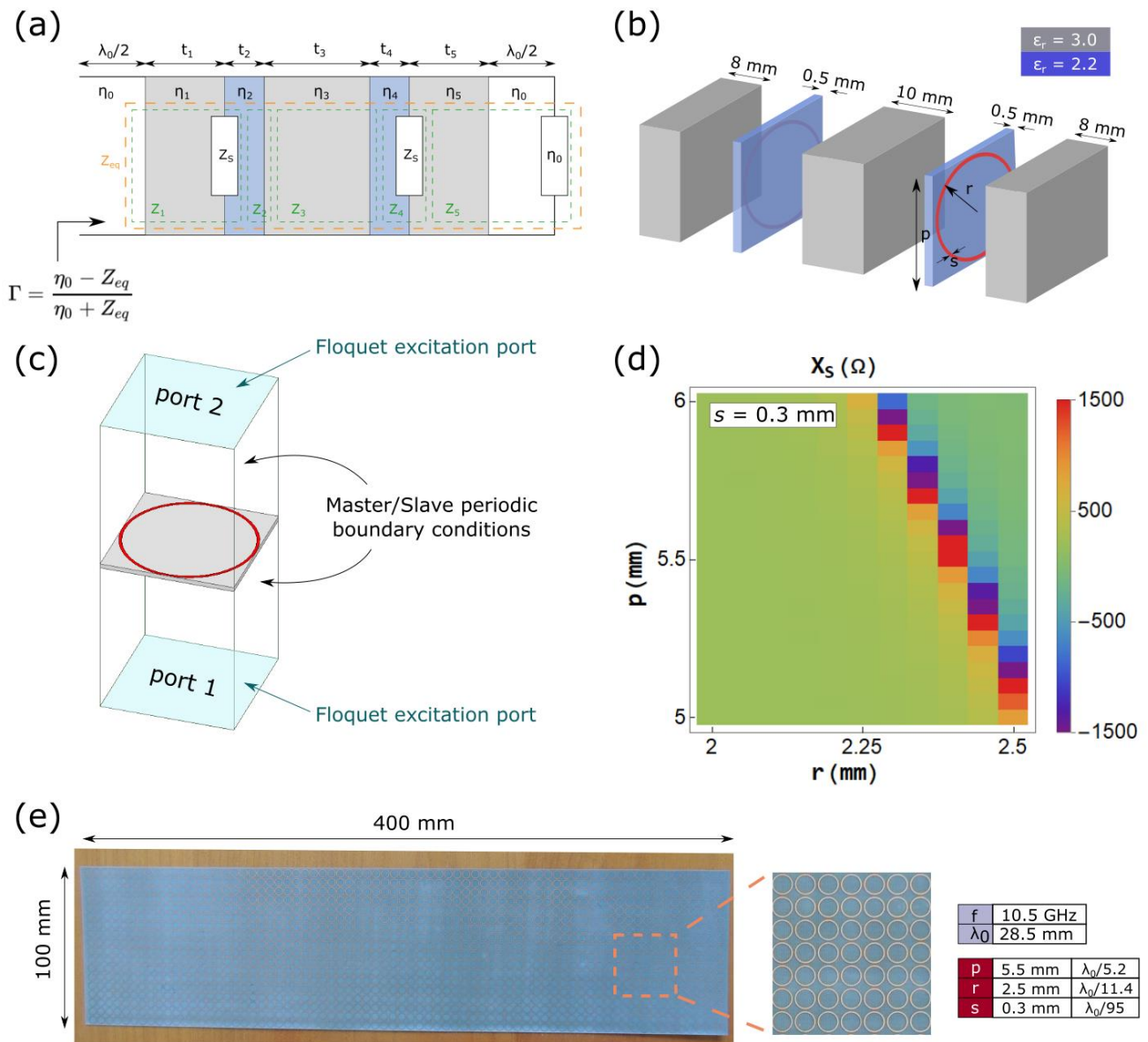
Figure 1. (a) Transmission line model of the metasurface-tuned seam. (b) Exploded view of a unit cell of the metasurface-tuned seam, comprising of three dielectric slabs ( \epsilon_r = 3.0 ) sandwiching two dielectric substrates ( \epsilon_r = 2.2 and \tan \delta = 0.001 ) onto which the meta-atoms are patterned. The ring meta-atom is characterized by its period p , outer radius r and width s . (c) Meta-atom's simulation setup. The ring meta-atom is simulated in a periodic environment using Master/Slave boundary conditions and excited by Floquet ports. (d) Evolution of the reactance of a circular ring unit-cell as a function of its period p and outer radius r at 10.5 GHz. (e) Photography of the fabricated metasurface using printed circuit board technique with a zoom view on the unit-cells and a table giving the optimized unit-cell parameters.
