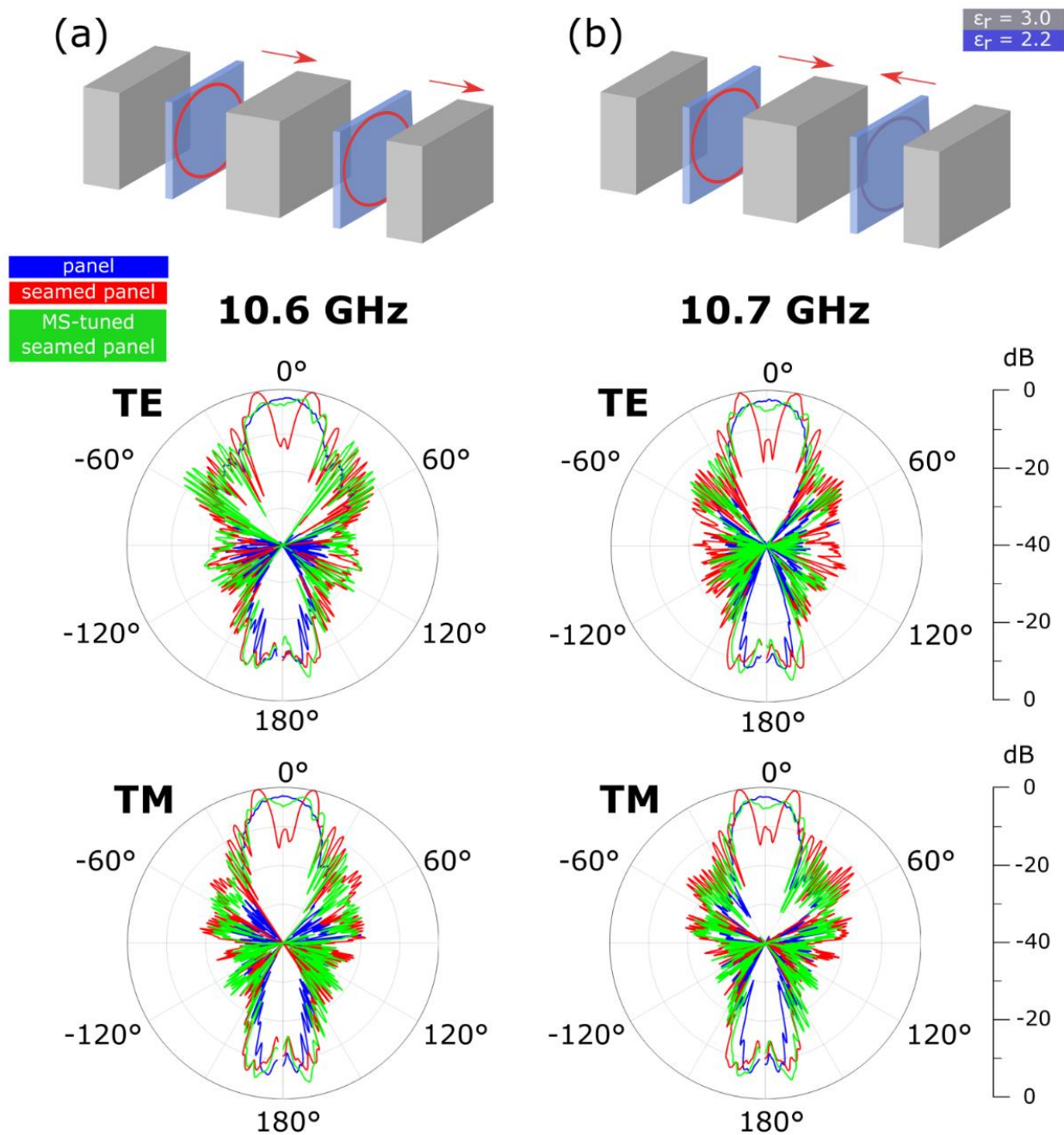
Figure 6. Variations of MS-tuned seam configuration and respective far-field radiation patterns. The red arrows in the schematic indicate the side of the substrate onto which the MS is patterned. (a) First variation: the first MS point inward and the second one outward. The scattering reduction effect is achieved at 10.6 GHz. (b) Second variation: both MS point inward. The scattering reduction effect is achieved at 10.7 GHz.
