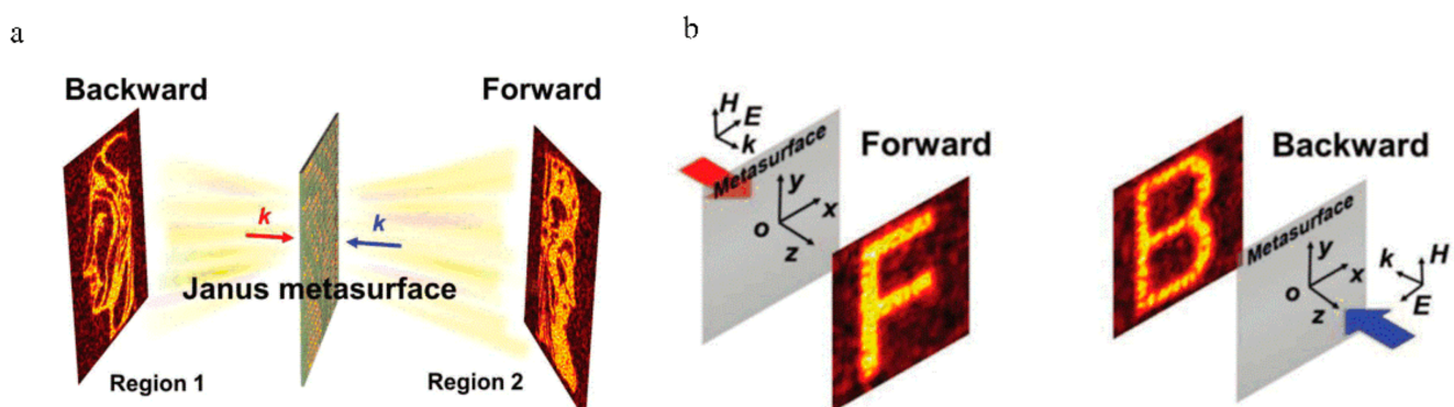
Figure 7. (a) Illustration of a Janus metasurface with bidirectional transmission for full-space wave manipulation. Adapted with permission from ref. [119]. Copyright 2019 John Wiley and Sons. (b) The incident wave forms different holograms for the two different propagation directions. Adapted with permission from ref. [119]. Copyright 2019 John Wiley and Sons.
