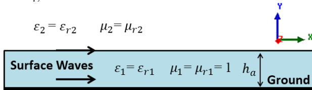
Fig. 1. Model of the grounded dielectric slab waveguide.
