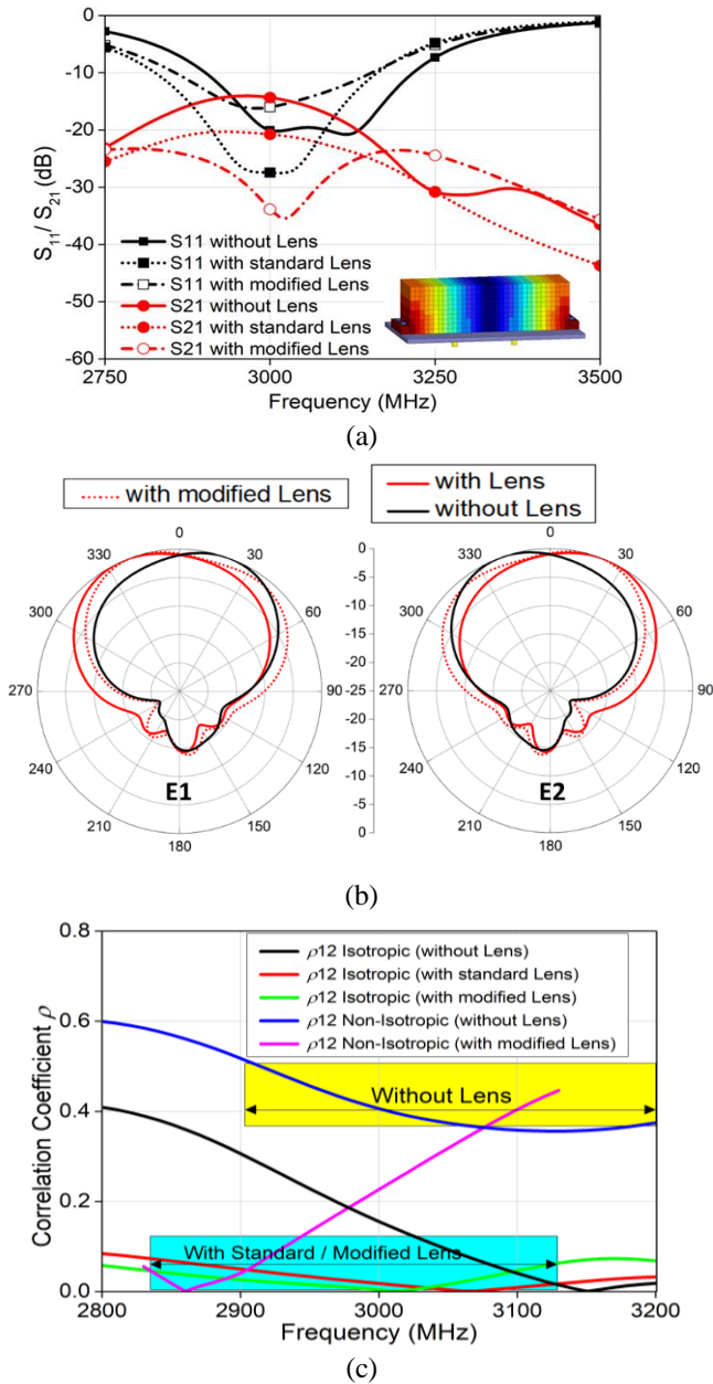
Fig. 4. Simulated results of 2-elements MIMO antenna with and without lens. (a) S -parameters. (b) Normalized radiation pattern E1 and E2 in the xoy -plane at 3 GHz. (c) Correlation coefficient.
