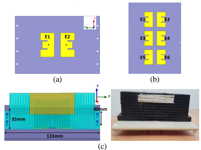
Fig. 12. (a) E-plane coupled 2-element E-patch MIMO antenna. (b) E-plane coupled 6-element E-patch MIMO antenna. (c) Geometry of the GID lens loaded 2-element MIMO antenna.
