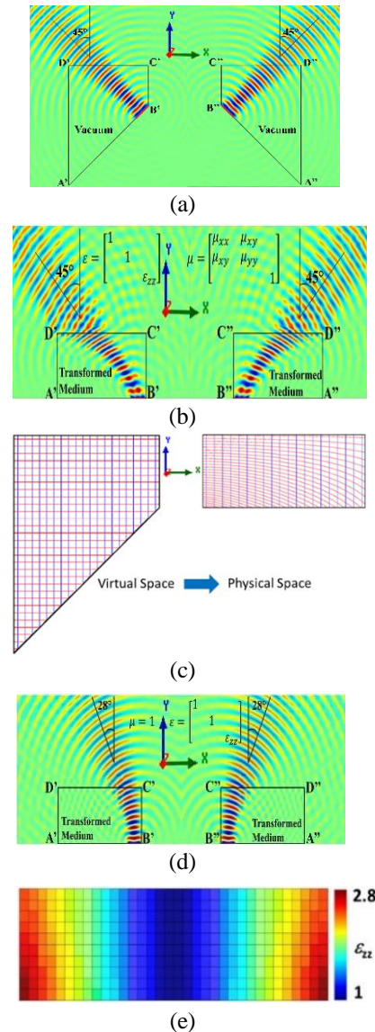
Fig. 5. Space mapping illustration. (a) Air-filled initial virtual space. (b) Calculated transformed ideal anisotropic lens. (c) QCTE mapping from virtual space to physical space. (d) Calculated simplified quasi-isotropic lens. (e) Permittivity ( \epsilon_{zz} ) profile of simplified quasi-isotropic lens.
