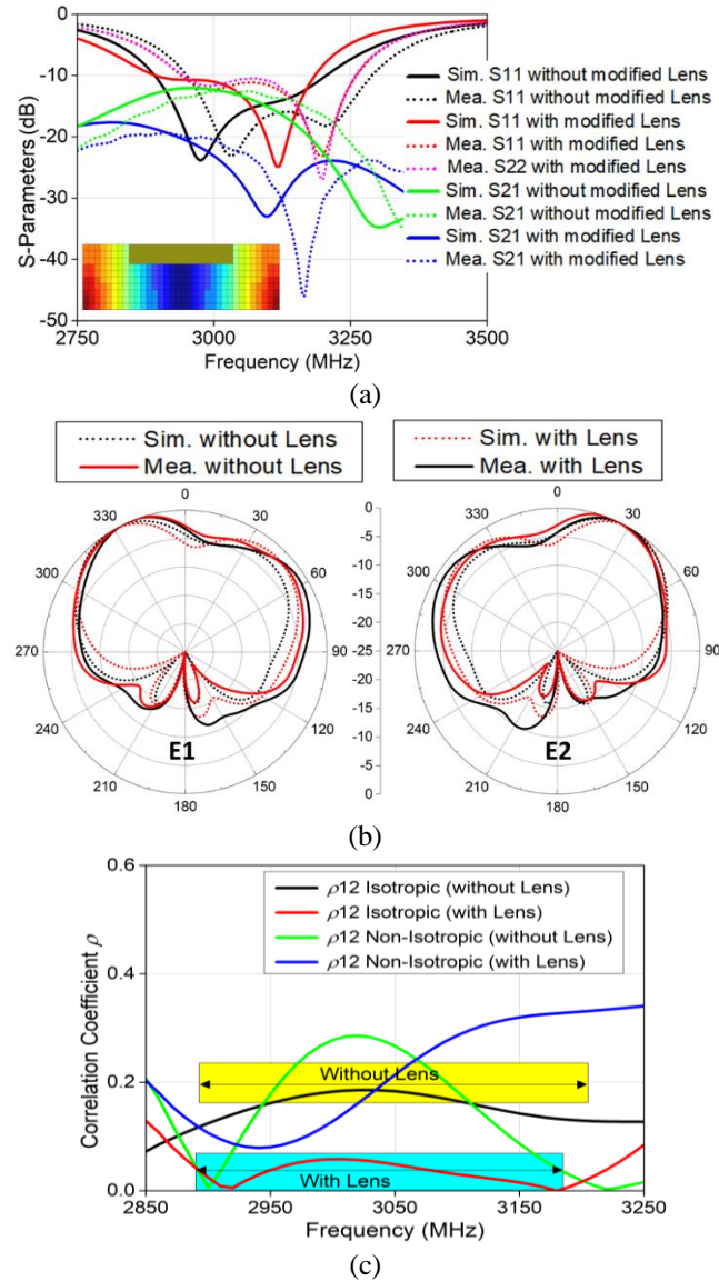
Fig. 13. Simulated and measured results of 2-elements E-plane coupled MIMO antenna with and without lens. (a) S-parameters. (b) Normalized radiation pattern E1 and E2 in the xy -plane. (c) Correlation coefficient.
