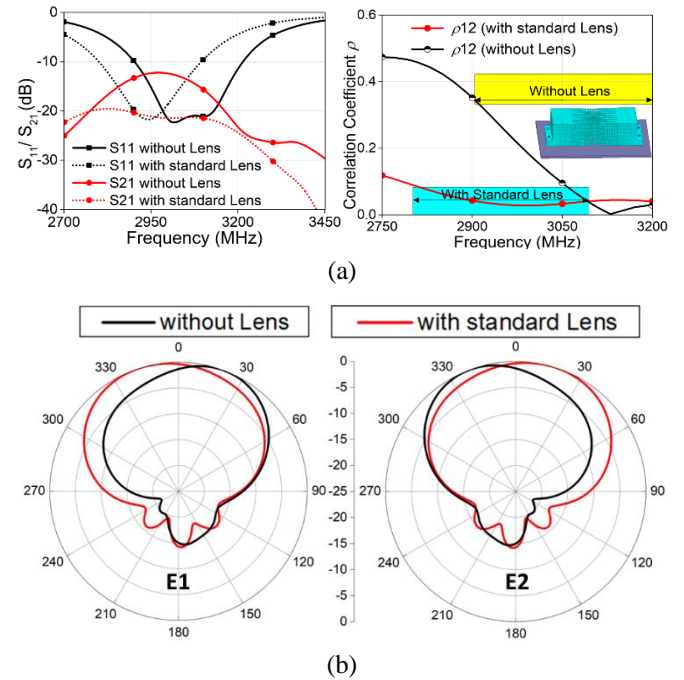
Fig. 8. Simulated results of 2-elements MIMO antenna with and without reduced unit cell size based PLA standard lens. (a) S -parameters and Correlation Coefficient. (b) Normalized radiation pattern E1 and E2 in the xoy -plane at 3 GHz.
