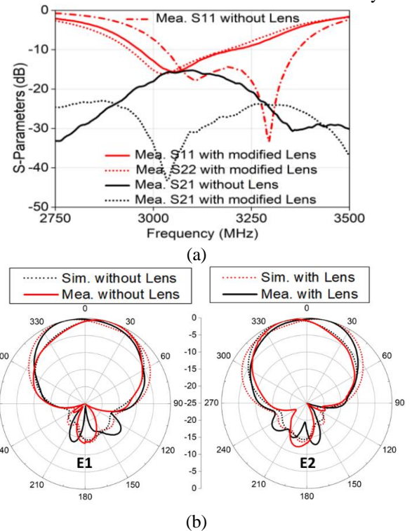
Fig. 10. Simulated and measured results of 2-element H-plane coupled MIMO antenna with and without lens. (a) S -parameters. (b) Normalized radiation pattern E1 and E2 in the xoy -plane.
