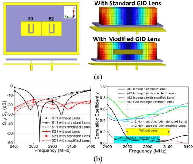
Fig. 16. (a) 2-element U-slot MIMO antenna with and without lens. (b) S-parameters and Correlation Coefficient.
