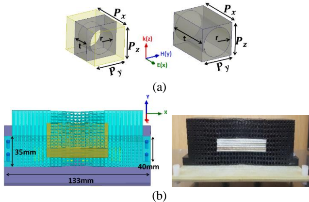
Fig. 7. (a) Dielectric unit cell for effective permittivity of 1.25 and 1.63, where P_x = 5 mm, P_y = P_z = 3.5 mm. (b) Geometry of the lens loaded 2-element H-plane decoupled MIMO antenna.
