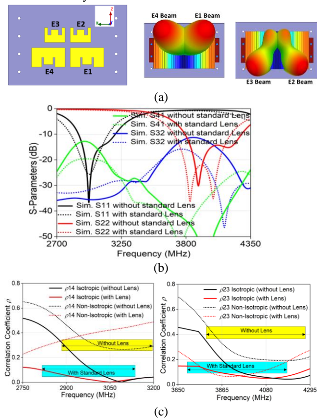
Fig. 15. (a) 4-element Multiband MIMO antenna with and without lens. (b) S -parameters. (c) Correlation Coefficient.
