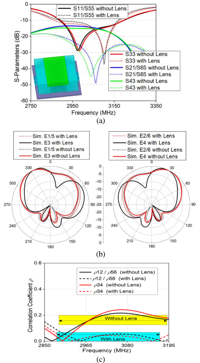
Fig. 14. Simulated results of 6-element MIMO antenna with and without lens. (a) S-parameters. (b) Normalized radiation pattern E1/ E3/ E5 and E2/ E4/ E6 in the xy -plane. (c) Correlation coefficient.
