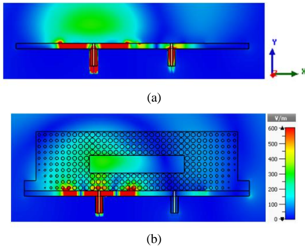
Fig. 11. E-field distribution of 2-element H-plane coupled MIMO antenna. (a) Without lens. (b) With lens.
