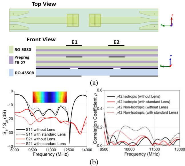
Fig. 17. (a) 2-element Stacked MIMO antenna with and without standard lens. (b) S-parameters and Correlation Coefficient.
