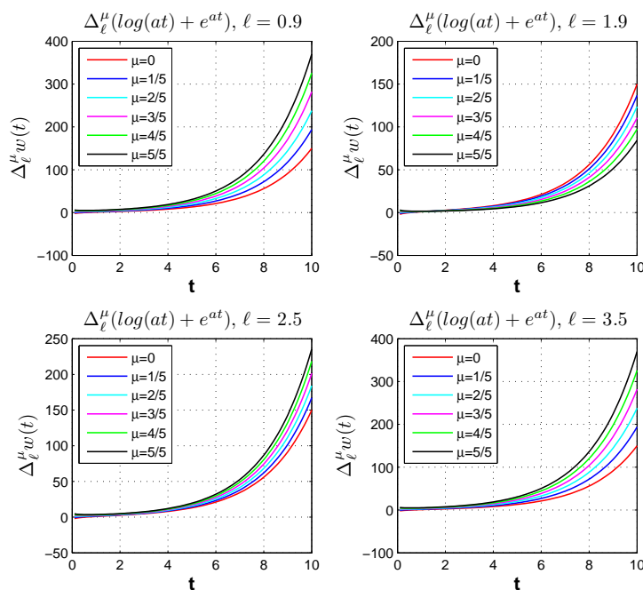
Figure 2. Generalized proportional difference of w(t) = \log(at) + e^{at} for different shift values \ell .
