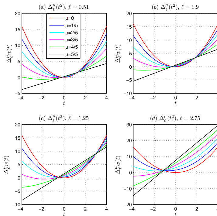
Figure 1. Generalized proportional difference of w(t) = t^2 for different shift values \ell .
