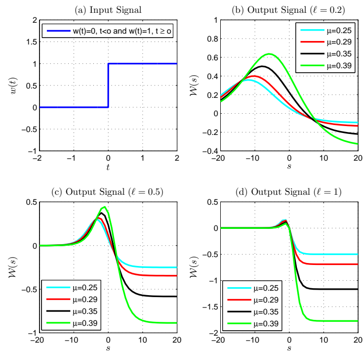
Figure 3. Generalized discrete proportional Laplace transform of the unit step function: (a) is the input signal, (b–d) show the output signal with fixed \ell (0.2, 0.5, and 1) and various \mu .
